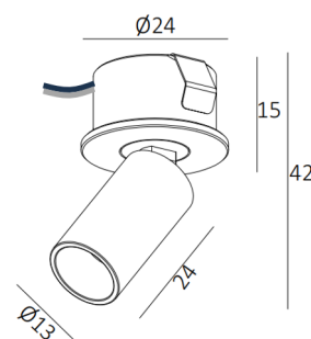
Cut-out 20mm
